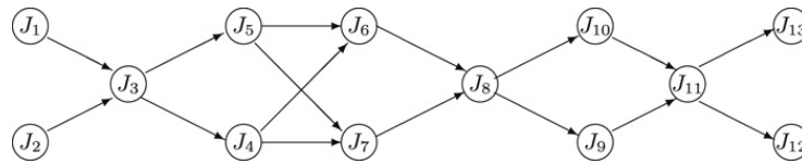
Fig. 2. Digraph G^0 = (\mathcal{J}, \mathcal{A}^0) constructed for Example 4.
