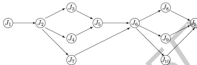
Fig. 1. Digraph G^0 = (\mathcal{J}, \mathcal{A}^0) constructed for Example 3.
