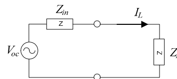
Figure 1. Equivalent circuit of antenna in receiving mode.
