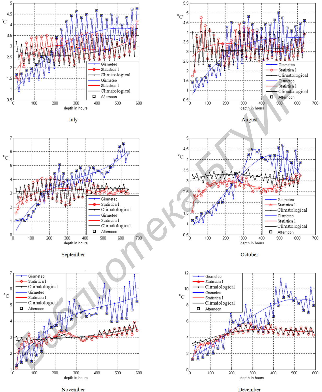
Figure 3. Graphs of a.m.e. of the monthly forecasts of the temperature (July – December).
