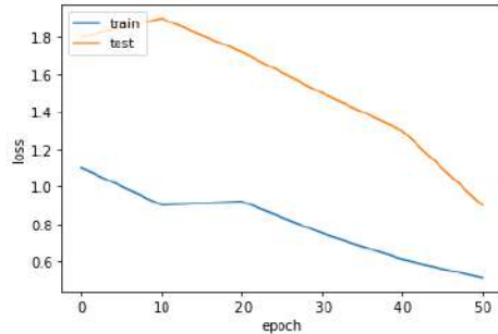
Figure 5. Model loss.
