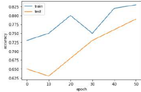
Figure 4. Model accuracy.
