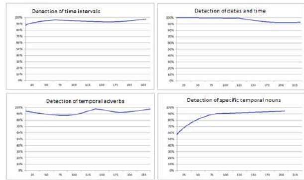
Figure 1. The results of experiments to detect temporal markers (the Oy axis is the percentage of detected markers of the total number, the Ox axis is the number of temporal markers)
