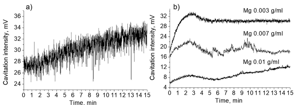
Fig. 9. Transient cavitation curves measured for water (a) and Mg aqueous suspensions (b) by hydrophone located under the sonotrode.
