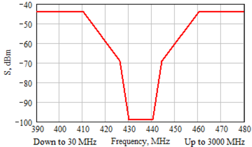
Fig. 2. Susceptibility to interference of SRD 1 receiver
