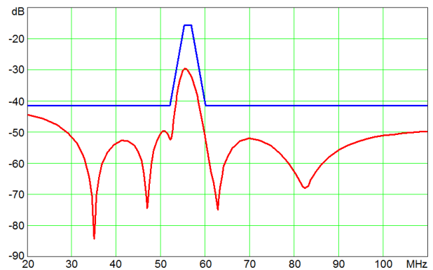
Fig 5 AFC of the SC through an antenna filter unit (AFU): blue line - pessimistic model based on data from technical specification; the red line is the refined model obtained from the measurement results
