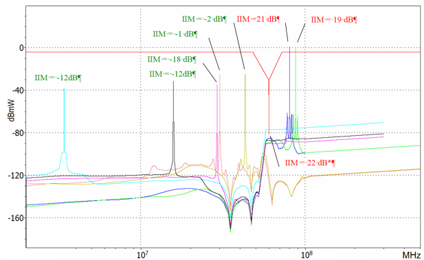
Fig 9 Results of the EMC DLA of CLRS using conditionally pessimistic models: red line - characteristic of receptor susceptibility (RR of VHF transceiver), lines of other colors - spectra of signals of RTs of HF and VHF transceivers at the antenna input of the receptor (An example)
