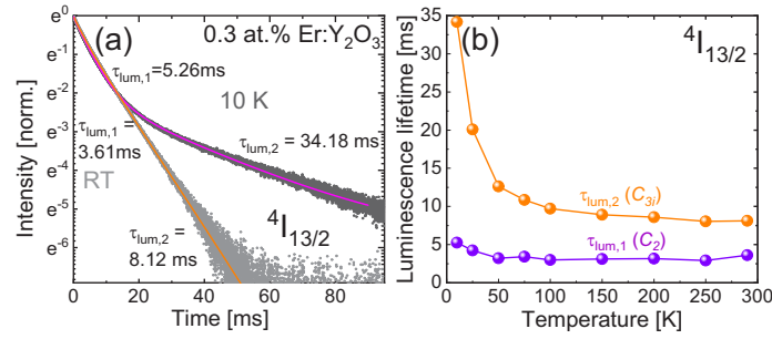
Fig. 7. Luminescence dynamics from the 4I_{13/2} state of Er^{3+} ions in 0.3 at.% Er:Y_2O_3 : (a) luminescence decay curves at RT and 10 K, the solid lines represent biexponential fits to the data, \lambda_{exc} = 1461 nm, \lambda_{lum} = 1543 nm; (b) temperature dependence of the ‘fast’ and ‘slow’ component of the biexponential fit.
