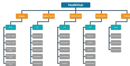
Fig. 2 Micro-Service structure for HIS system
