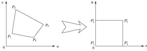
Fig. 4 Inverse perspective transformation
