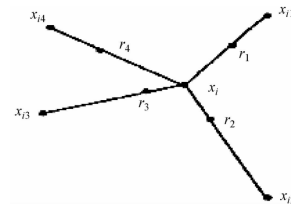
Fig. 1 Schematic diagram of SMOTE synthesis
