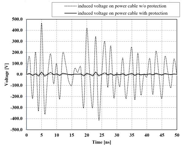
Fig. 9. Induced voltage measured on ECU power cable with protection.
