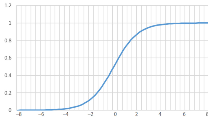
Figure 1. The graph of the logistic function.
