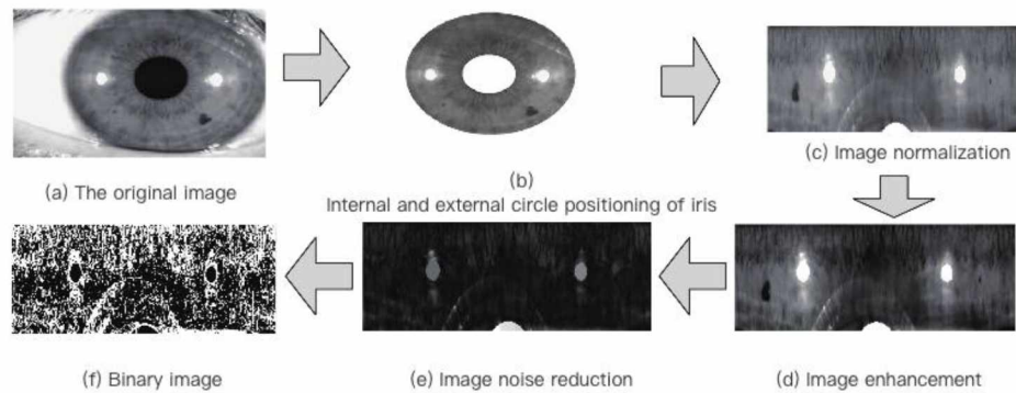
Figure 2 – Extraction process
